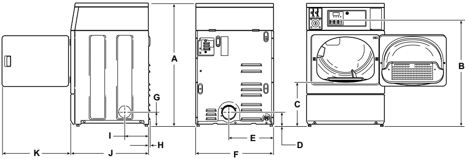
CDC10 Side CDC10 Back CDC10 Front
